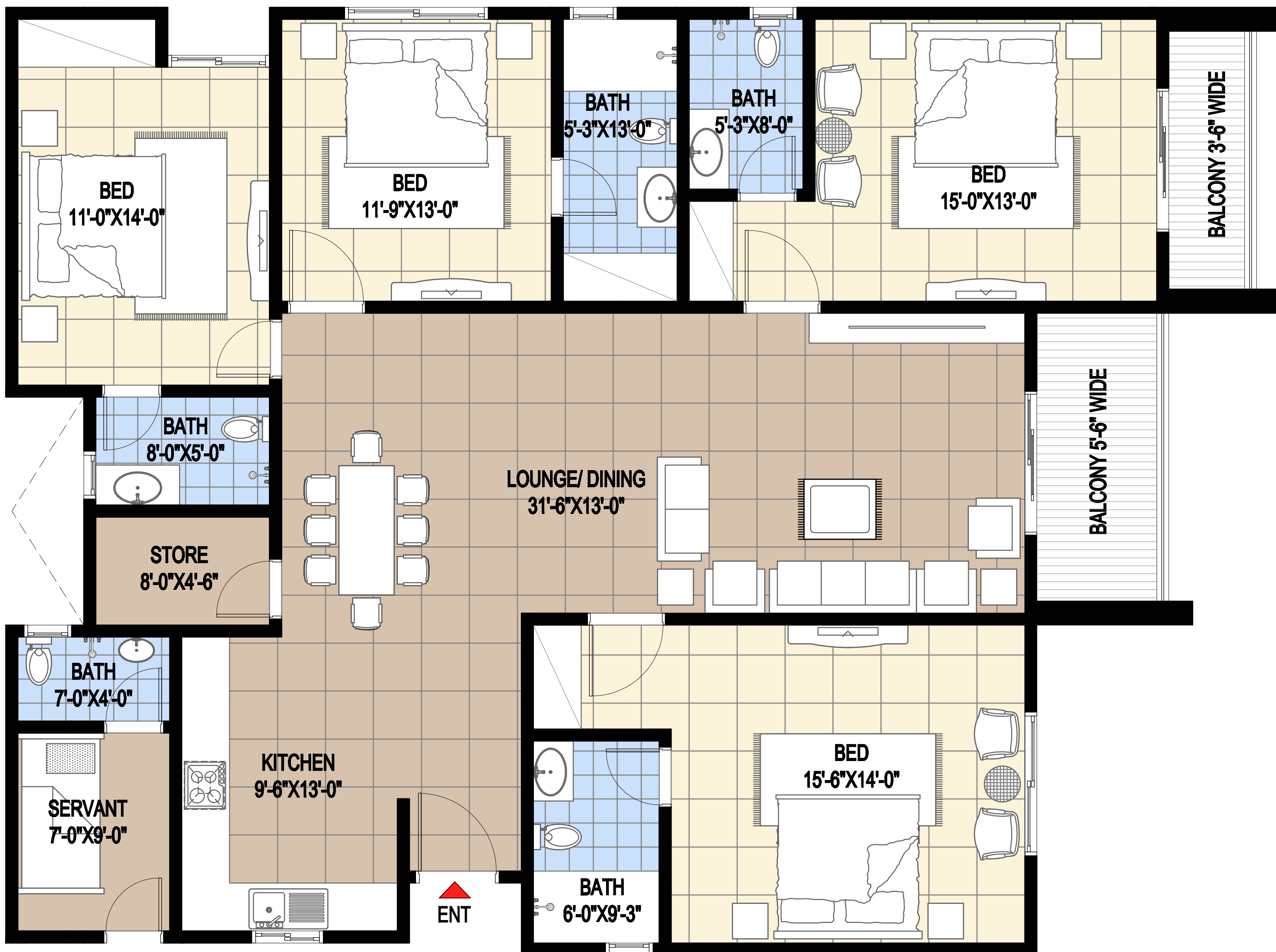
TYPE A GROSS AREA = 2550.00 SQ.FT
