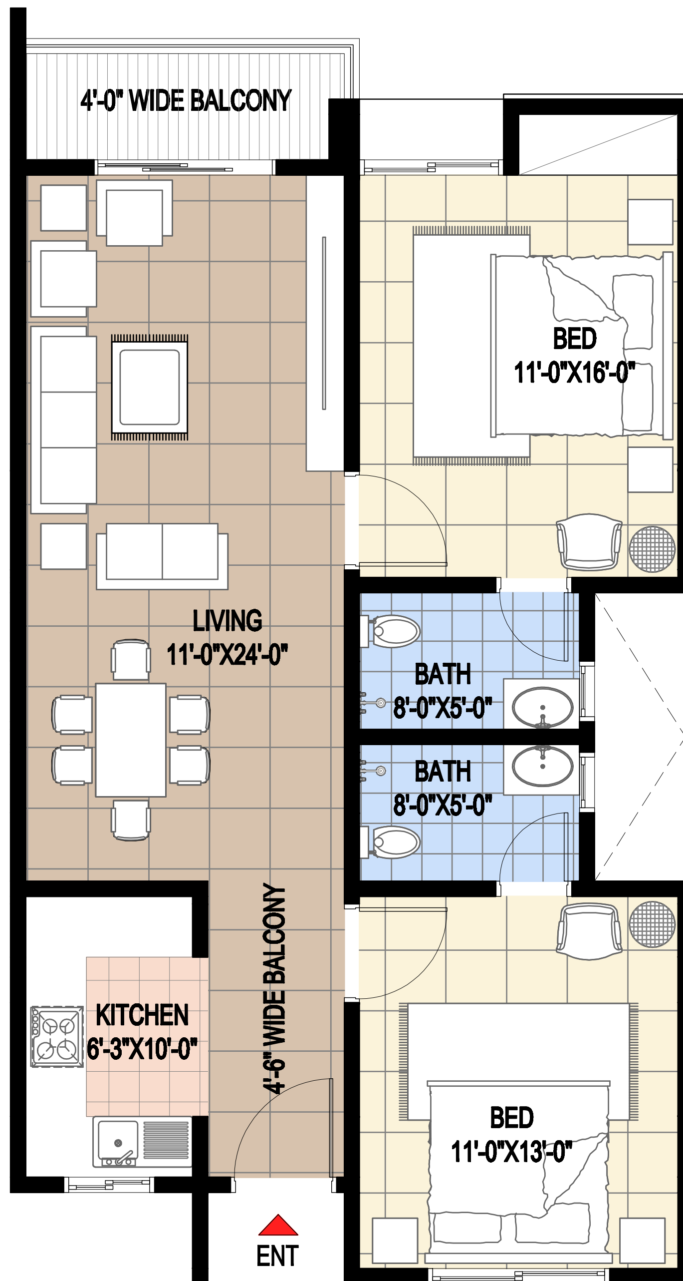
TYPE C GROSS AREA = 1198.00 SQ.FT
